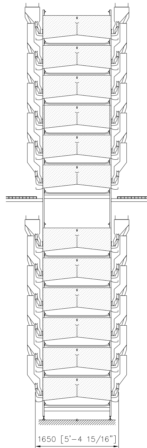
FRONT VIEW
